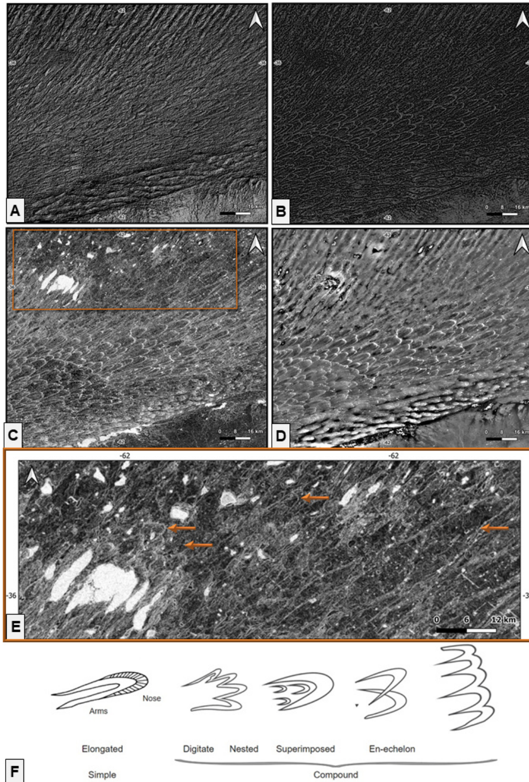
Figure 3. Application of the local entropy method to the CPD aeolian unit (Zone 1 in Fig. 1), where parabolic dunes were previously documented (Tripaldi et al. , 2025, and references therein). a) Standard hillshade model (azimuth 315°). Aeolian features are faint and poorly defined. b) Sky-view factor (SVF) map; features remain difficult to perceive. c) Local entropy map ( r = 2 pixels, \delta = 0.5 m). Dune ridges (white arrows) are sharply enhanced, with clear textural contrast between crests (high entropy) and interdune plains (low entropy). d) Simple local relief (SLR) model; dune boundaries are also visible, though with a different textural emphasis. e) Detail of a sector of the local entropy map (c) to illustrate how the linear pattern closes in a hook, which are interpreted as the arms and noses of parabolic dunes, respectively. f) Sketches of the different types of parabolic dunes recognized in the study areas (after Pye, 1993). This result demonstrates the method’s efficacy in highlighting subtle organized morphologies.
